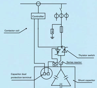
Combination Switching/Thyristor Switching Way
